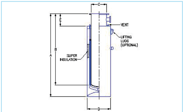
MAGNET DEWARs
